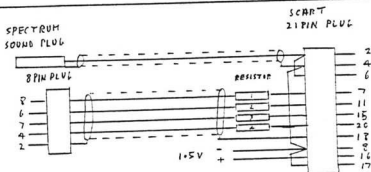
RESISTORS 1, 2 & 3 = 1000 OHM RESISTOR 4 = 1300 OHM.
